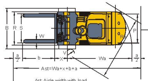
Ast: Aisle width with load a: Clearance b: Load Length
